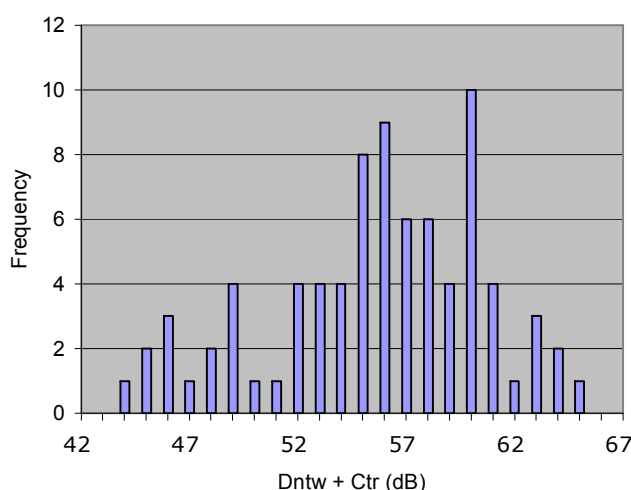
Figure 4 – Spread of results ( D_{nTw} + C_{tr} ) for the Timber Wall.
