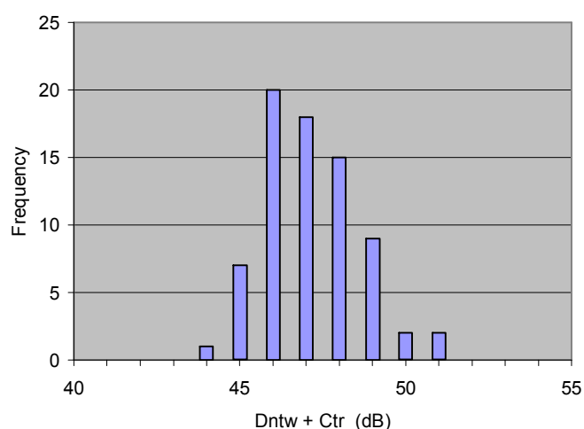
Figure 2 – Spread of results ( D_{nTw} + C_{tr} ) for the Concrete Floor.
