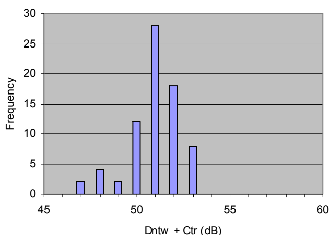
Figure 1 – Spread of results ( D_{nTw} + C_{tr} ) for the Masonry Wall.
