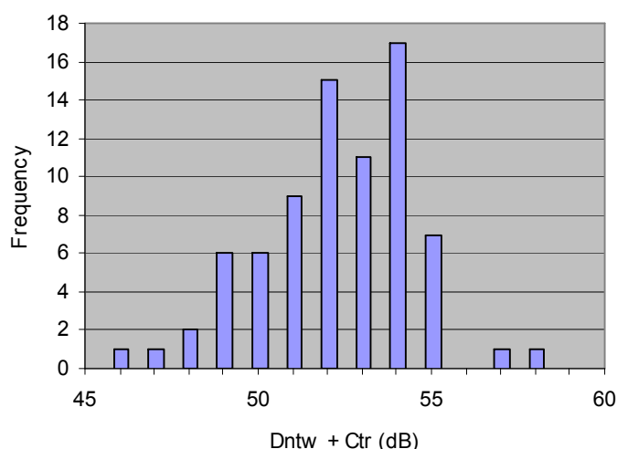
Figure 3 – Spread of results ( D_{nTw} + C_{tr} ) for the Timber Floor.
